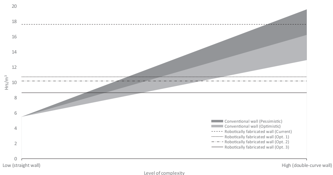
Fig. 13. Productivity (h/m 3 ) for different levels of complexity for a concrete wall using conventional construction and robotic fabrication.
